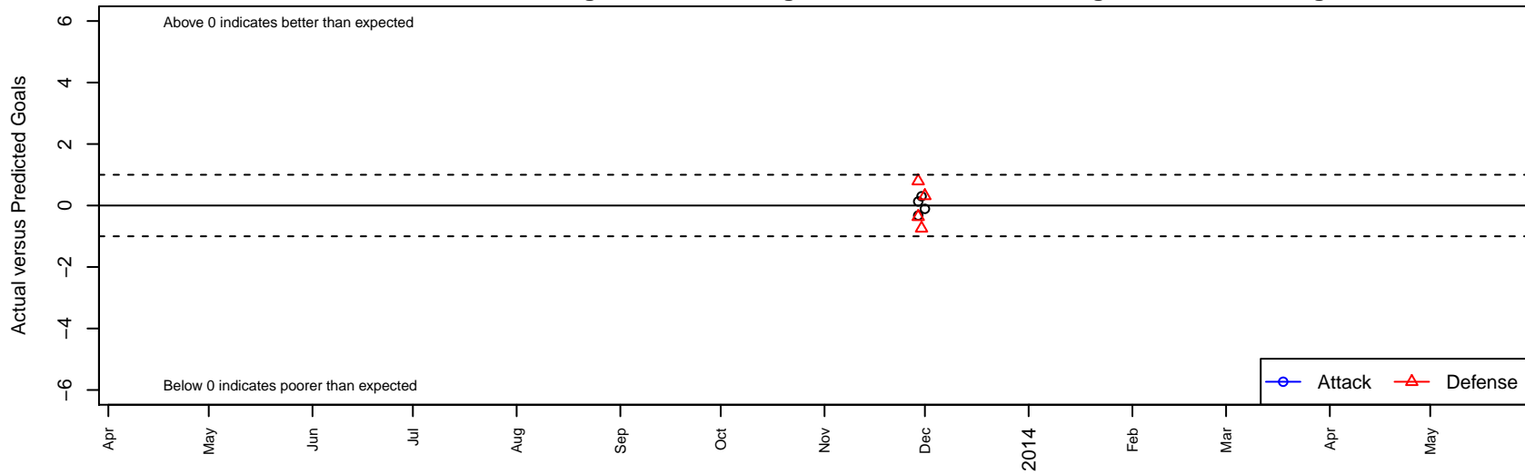
Milan FC Black B97 Dots are actual minus expected GF (blue circles) and GA (red triangles). Blue line is smoothed change in attack strength. Red is smoothed change in defense strength.
